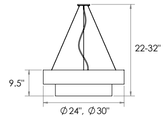
CC3 suspension
